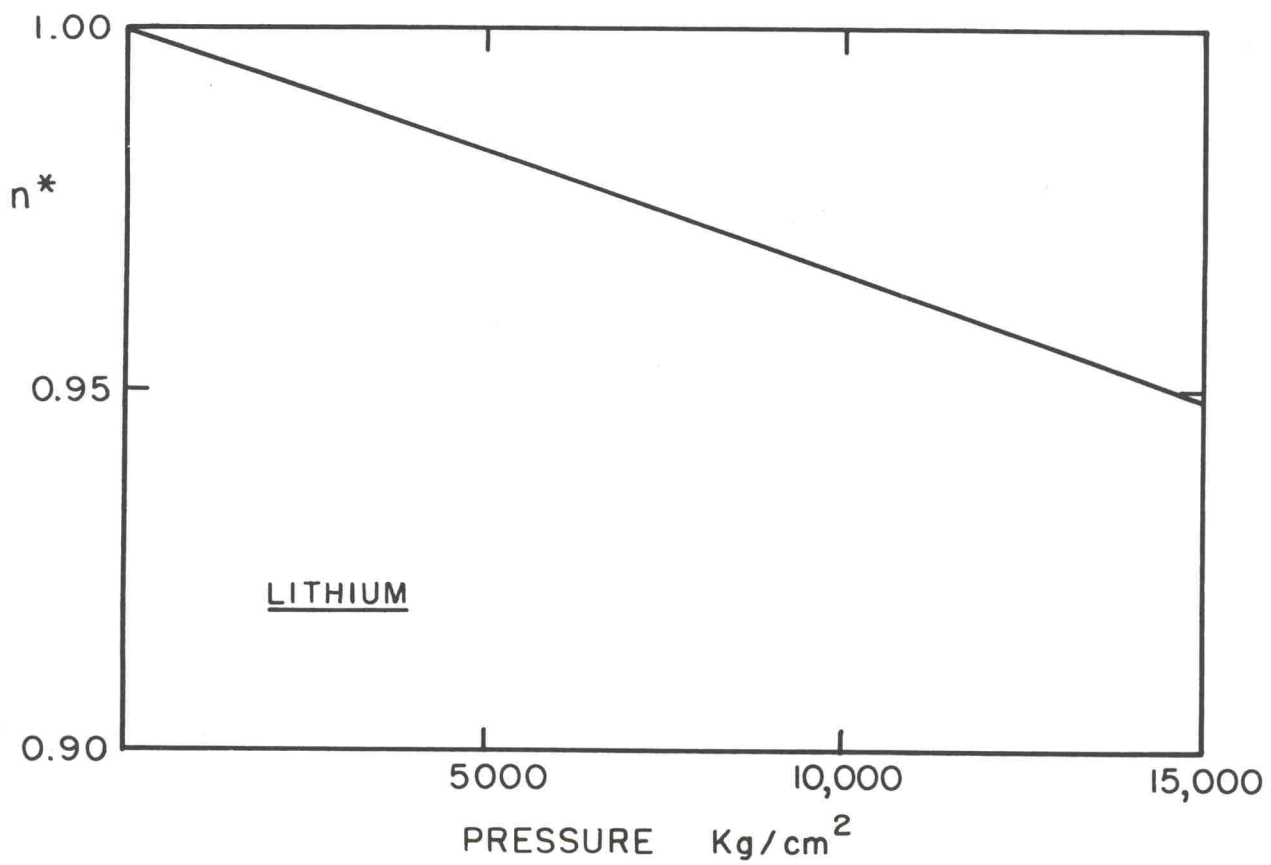
FIG. 3-10 n^* , NORMALIZED ELECTRONS/ATOM VS. PRESSURE
